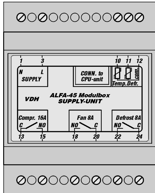
SUPPLY-unit
